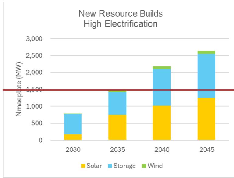
Figure 24: Resource Additions under High Electrification Load Forecast
