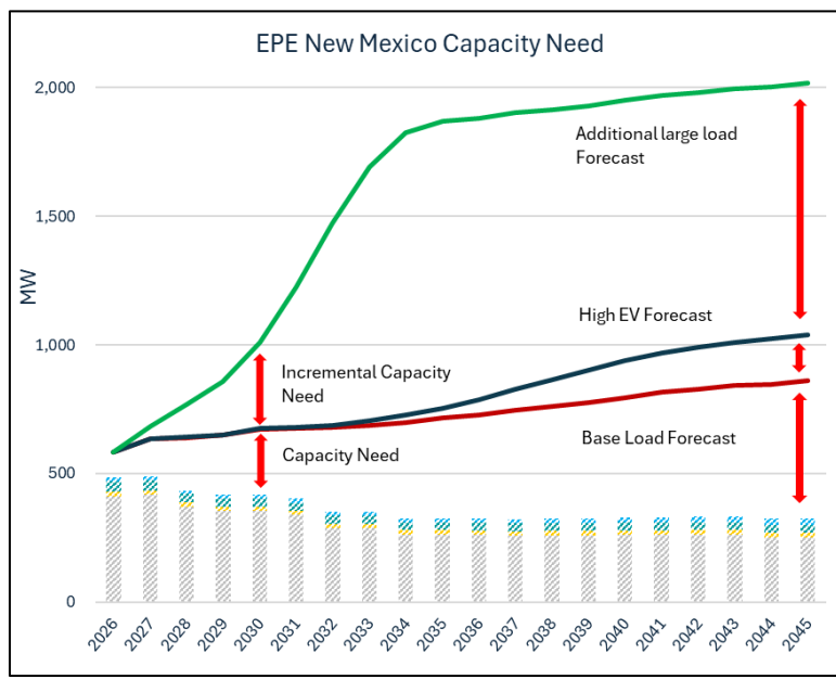
Figure 1: EPE New Mexico Capacity Need
