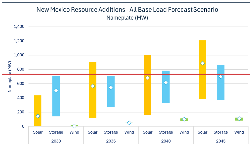
Figure 43: Resource Additions under Conservative Base Load Forecast
